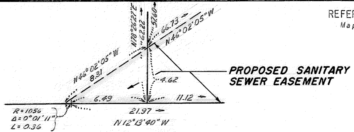
DETAIL "A"
